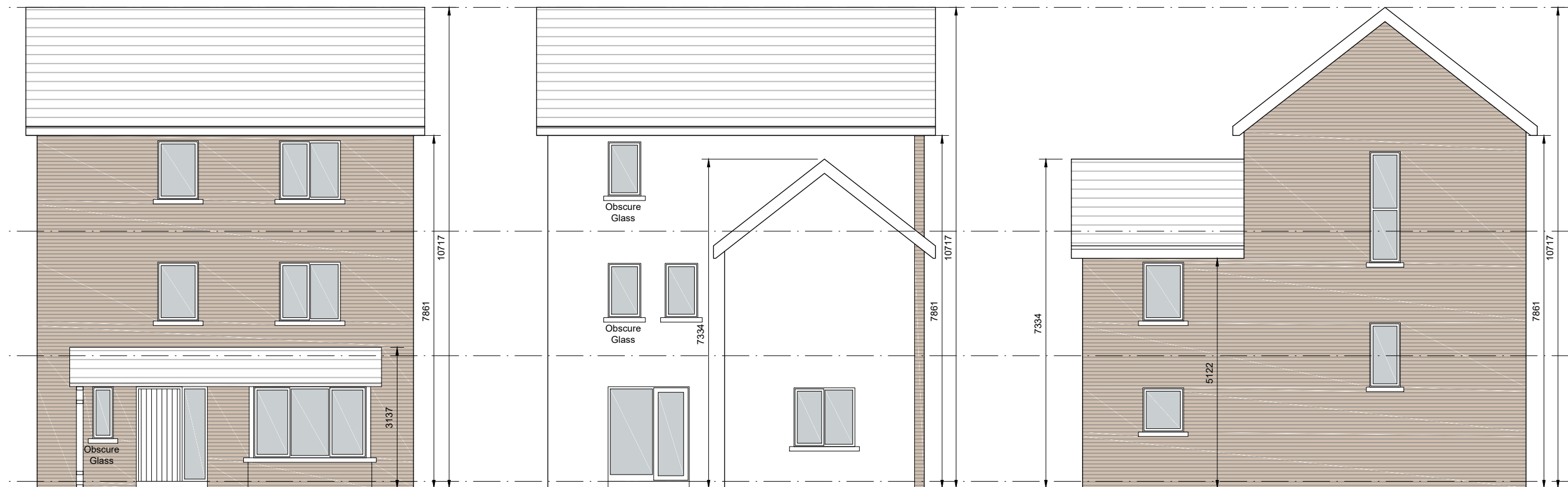
SOUTH ELEVATION
